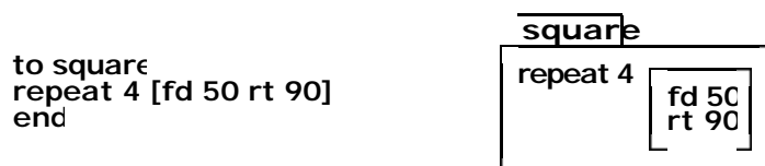
Figure 1. A square procedure definition in Logo (left) versus a visually transparent Boxer presentation (right).
