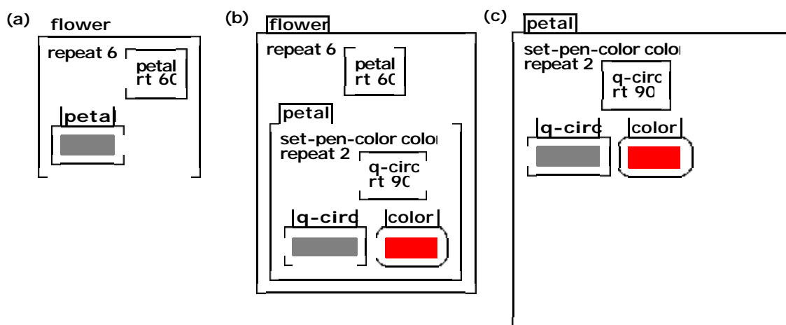
Figure 4. (a): A procedure contains a subprocedure, which is shrunk to hide its details. (b): Clicking on the subprocedure opens it to reveal its contents. (c): If the contents are complex, the user can click to expand the subprocedure to full-screen size. A click to shrink the box brings one back to (b).
