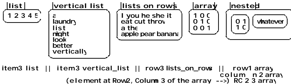
Figure 5. Some different arrangements of Boxer data and, below each, Boxer expressions selecting a part of the data.
